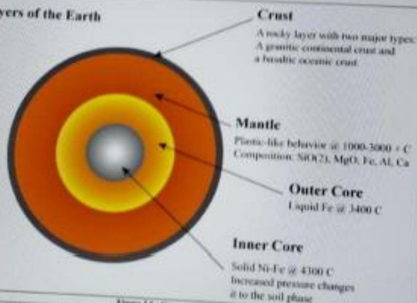
Figure 3.1 : Cross section of Earth
